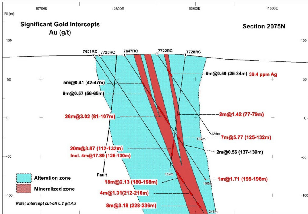
Figure 2: Cross section line 2075N, showing significant Au intercepts.
