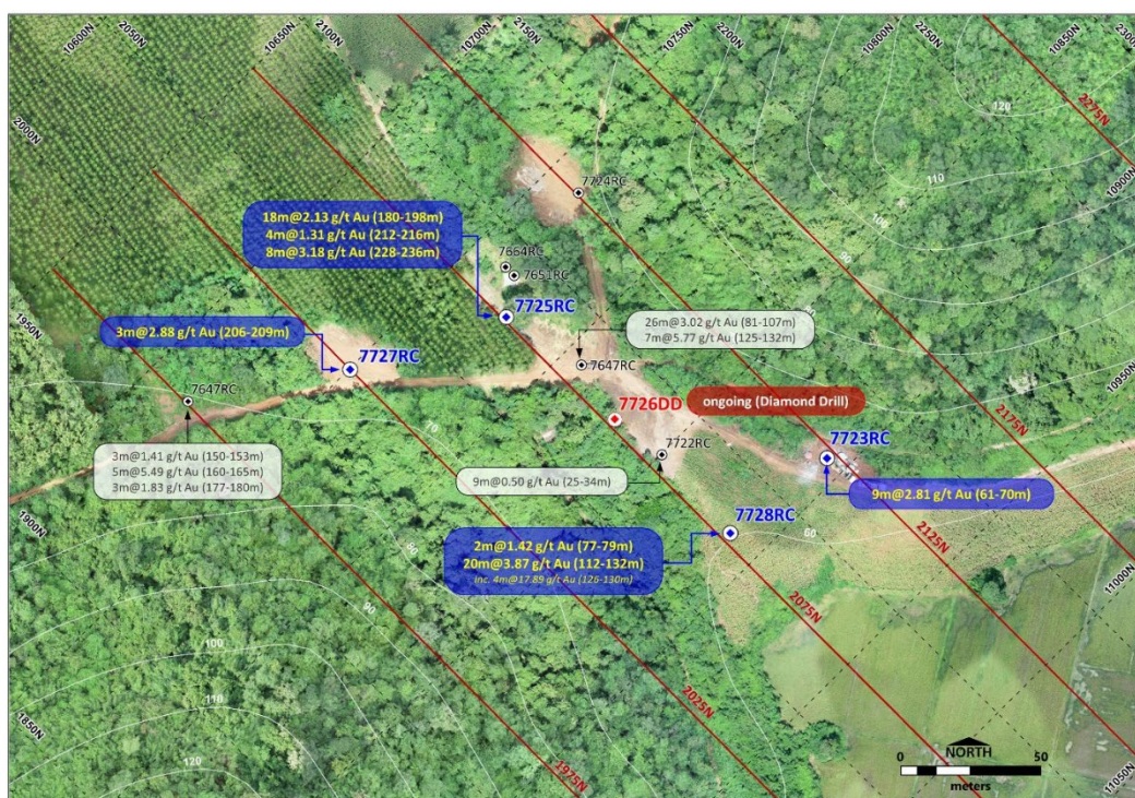
Figure 1: Drill hole locations and assay highlight in the middle zone (section 2025N, 2075N and 2125N).
